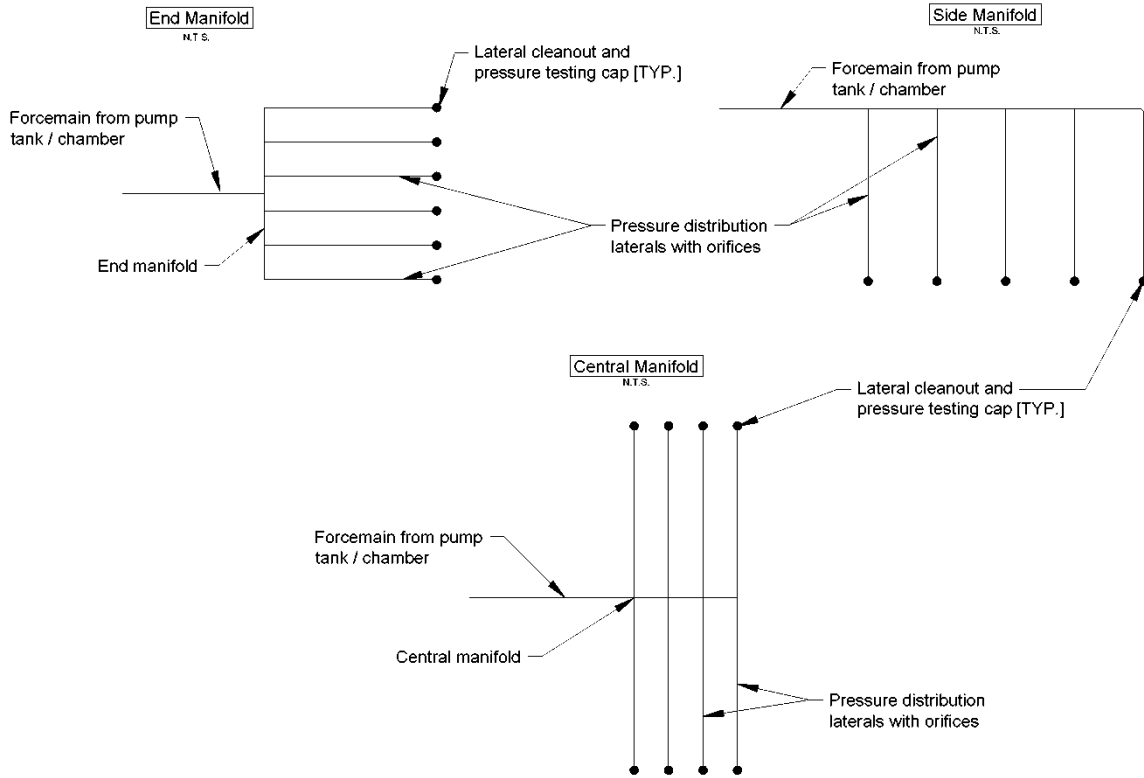
Pressurized Flow Splitting Configurations
