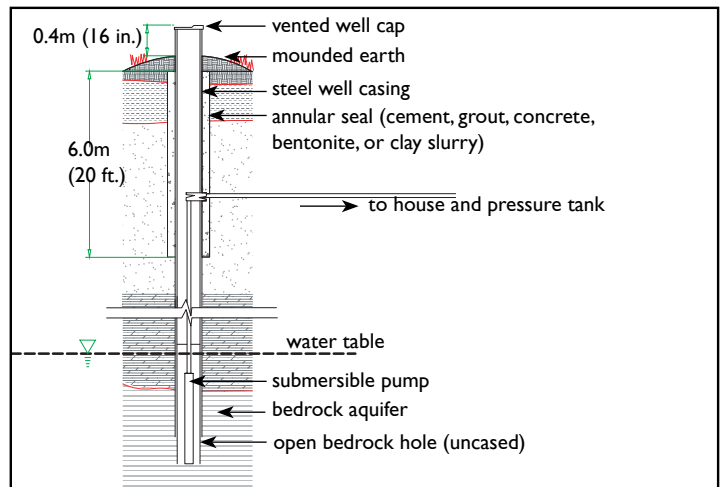
Figure 2: Drilled Well
