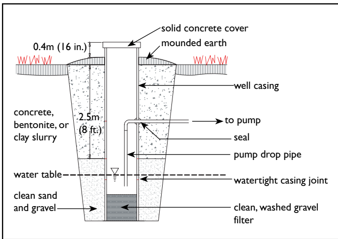
Figure 1: Dug Well
